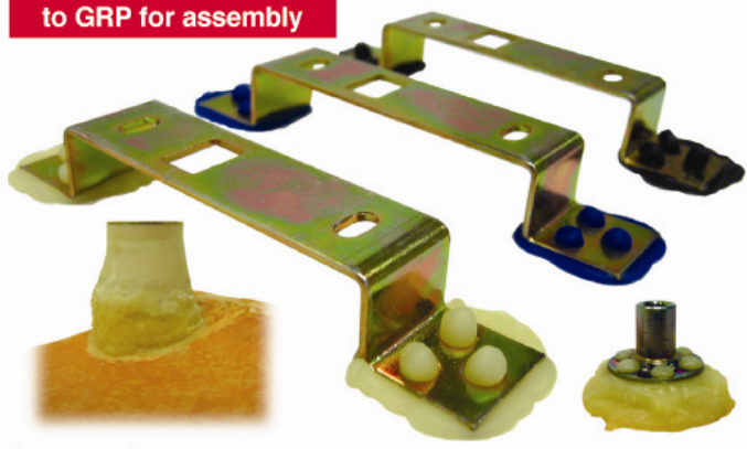
Different fixings bonded to GRP for assembly
